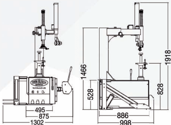
(1) Help-arm for professional use (2) Mounting head (3) Comfortable and clear tire inflator (4) Self centering wheel mounting system (5) Wheel lifter
